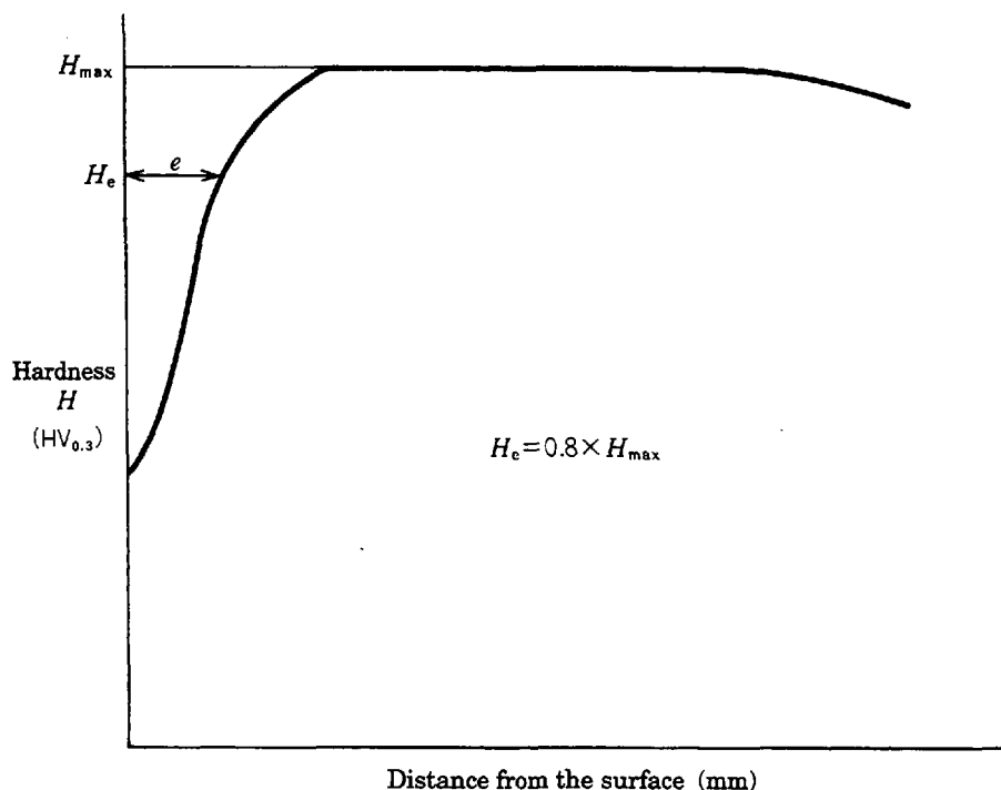
Figure 2 Determination of the depth of the decarburized zone
