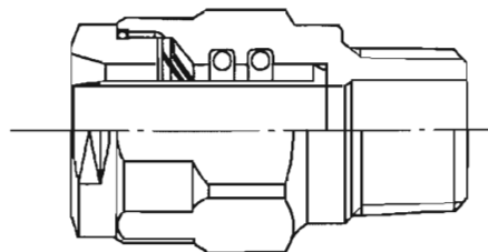
e) Fitting used to secure water-tightness with an O-ring by fixing a pipe by holding ring
