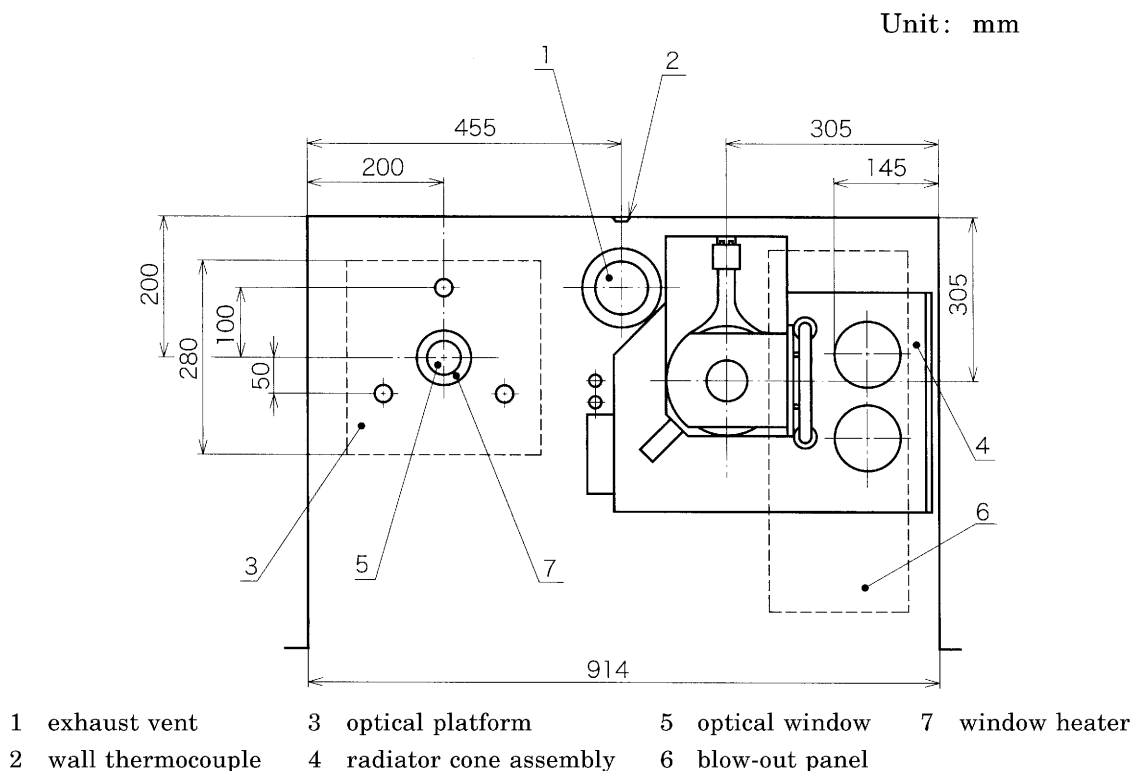
Figure 2 Plan view of typical chamber
