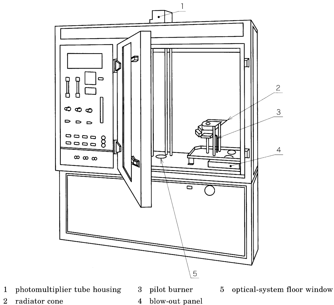
Figure 1 Typical arrangement of test apparatus
