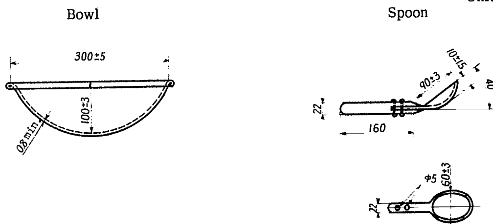
Fig. 1. Dimensions of bowl and spoon
