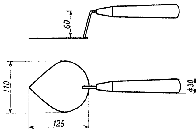
Fig. 2. An example of dimensions of trowel
