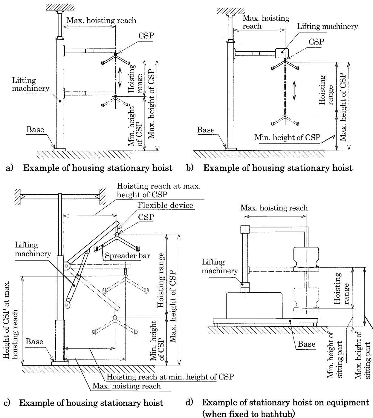
Figure 1 Example of stationary hoist (Hoisting range/reach)
