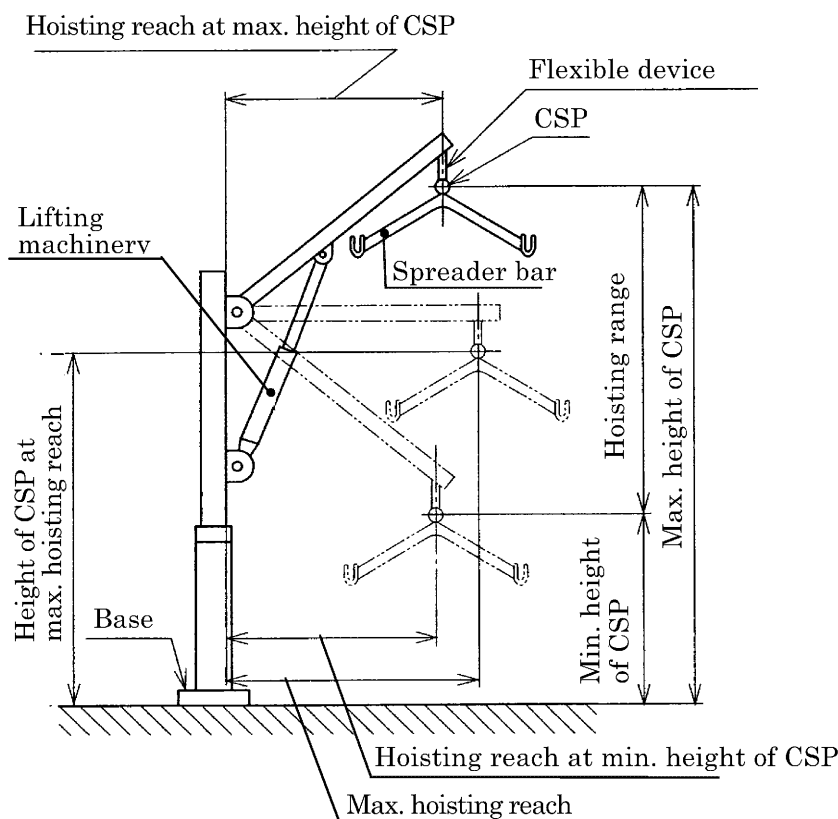
e) Example of stationary hoist on equipment
