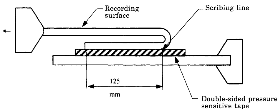
Figure 1 Measurement of the coating adhesion
