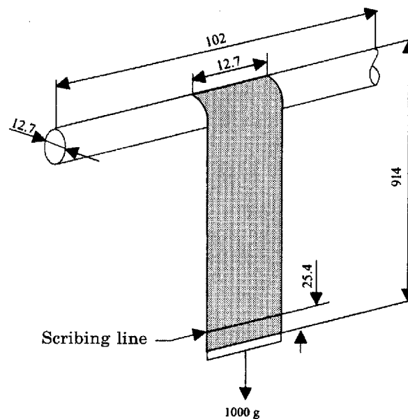
Figure 2 Measurement of layer-to-layer adhesion
