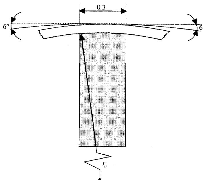
Figure 4 Measurement of abrasivity (not to scale)
