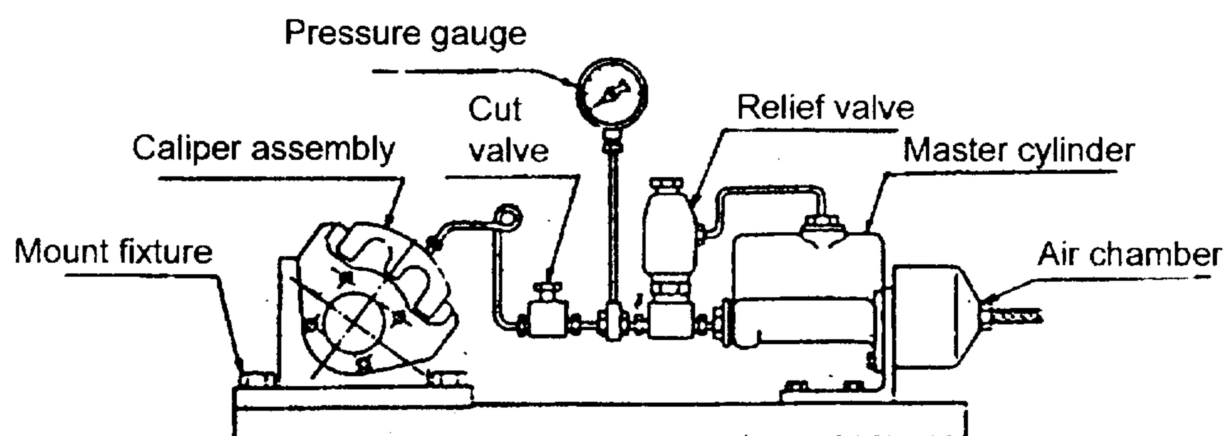
Fig. 1 Pressing equipment
