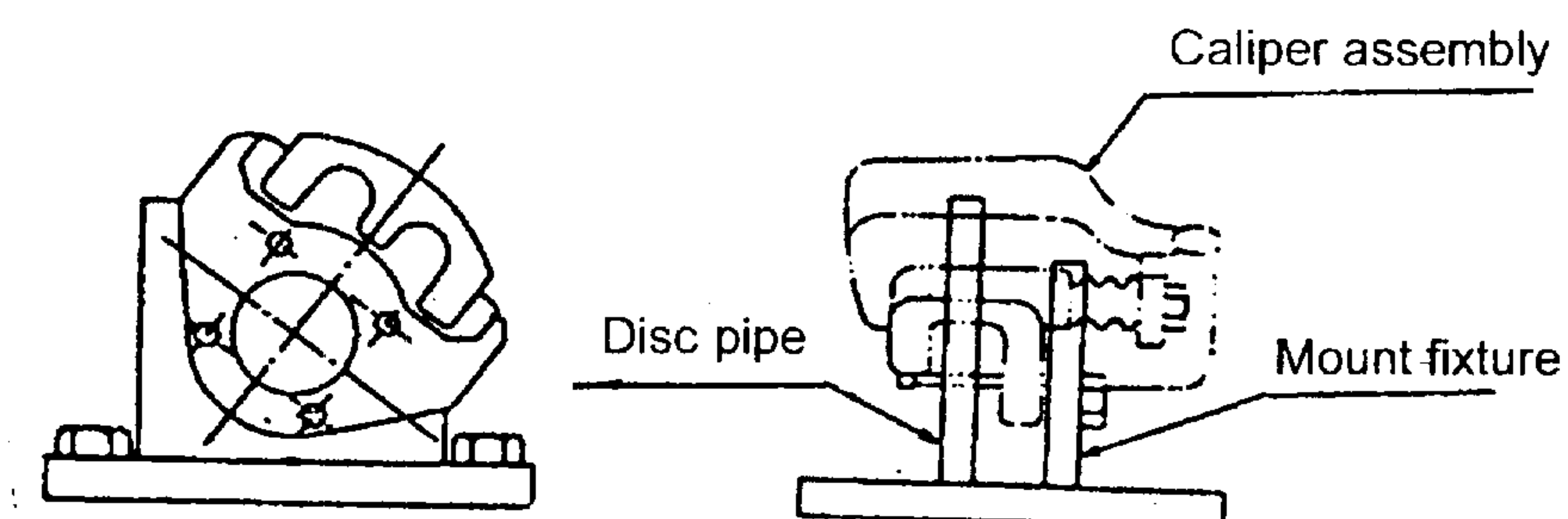
Fig. 2 Mount fixture
