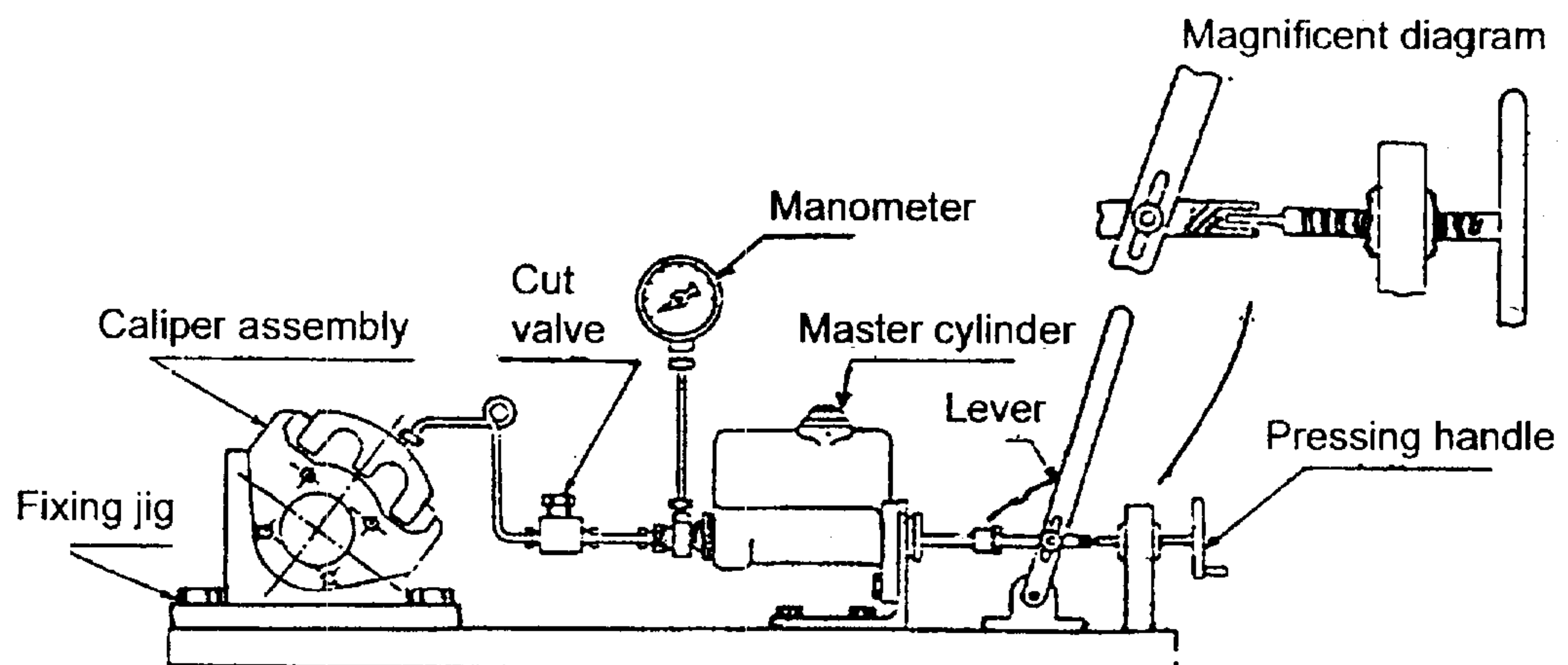
Fig. 1 Example of manual pressing unit
