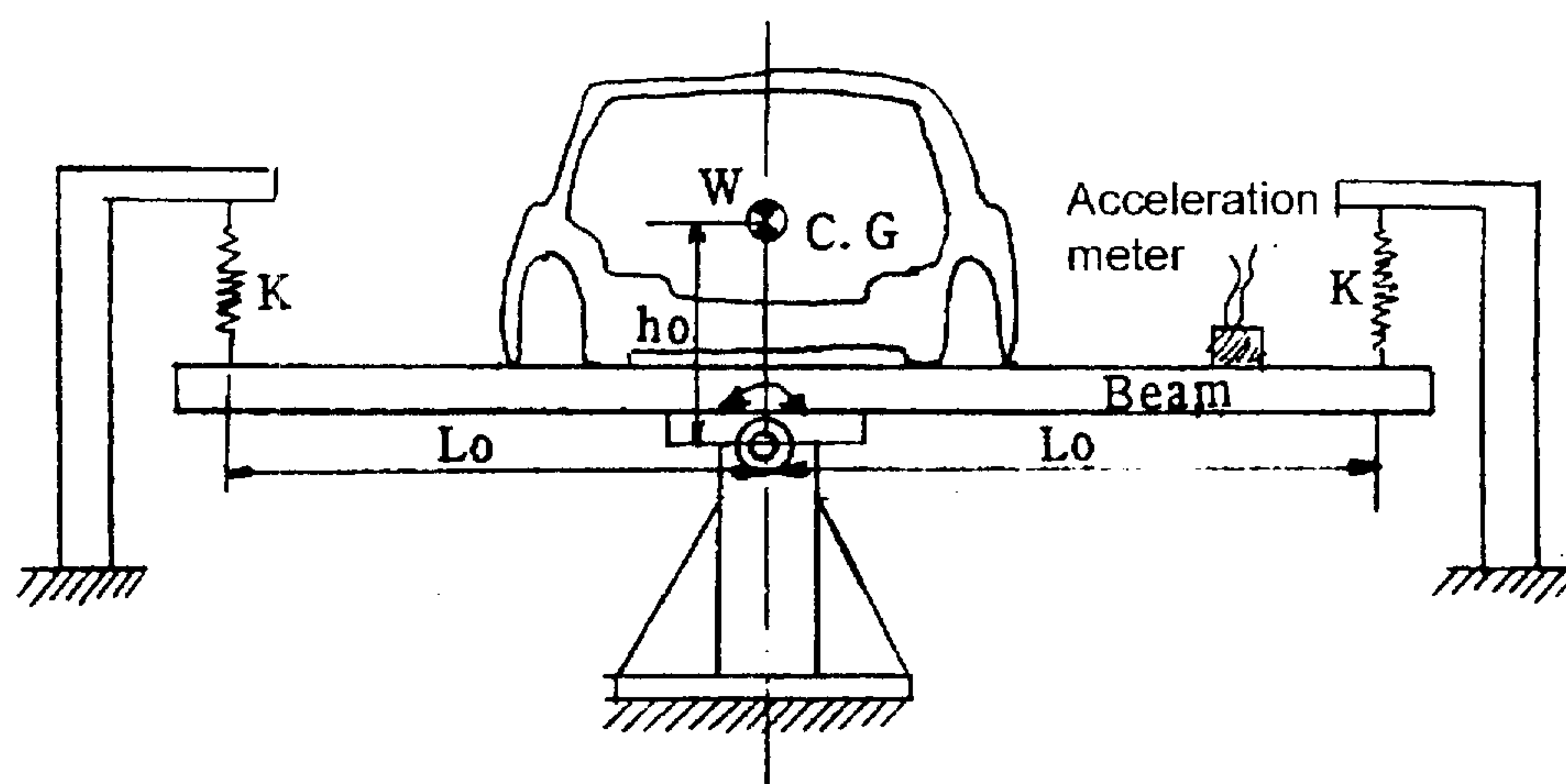
Figure 1. Outline Drawing of Test
