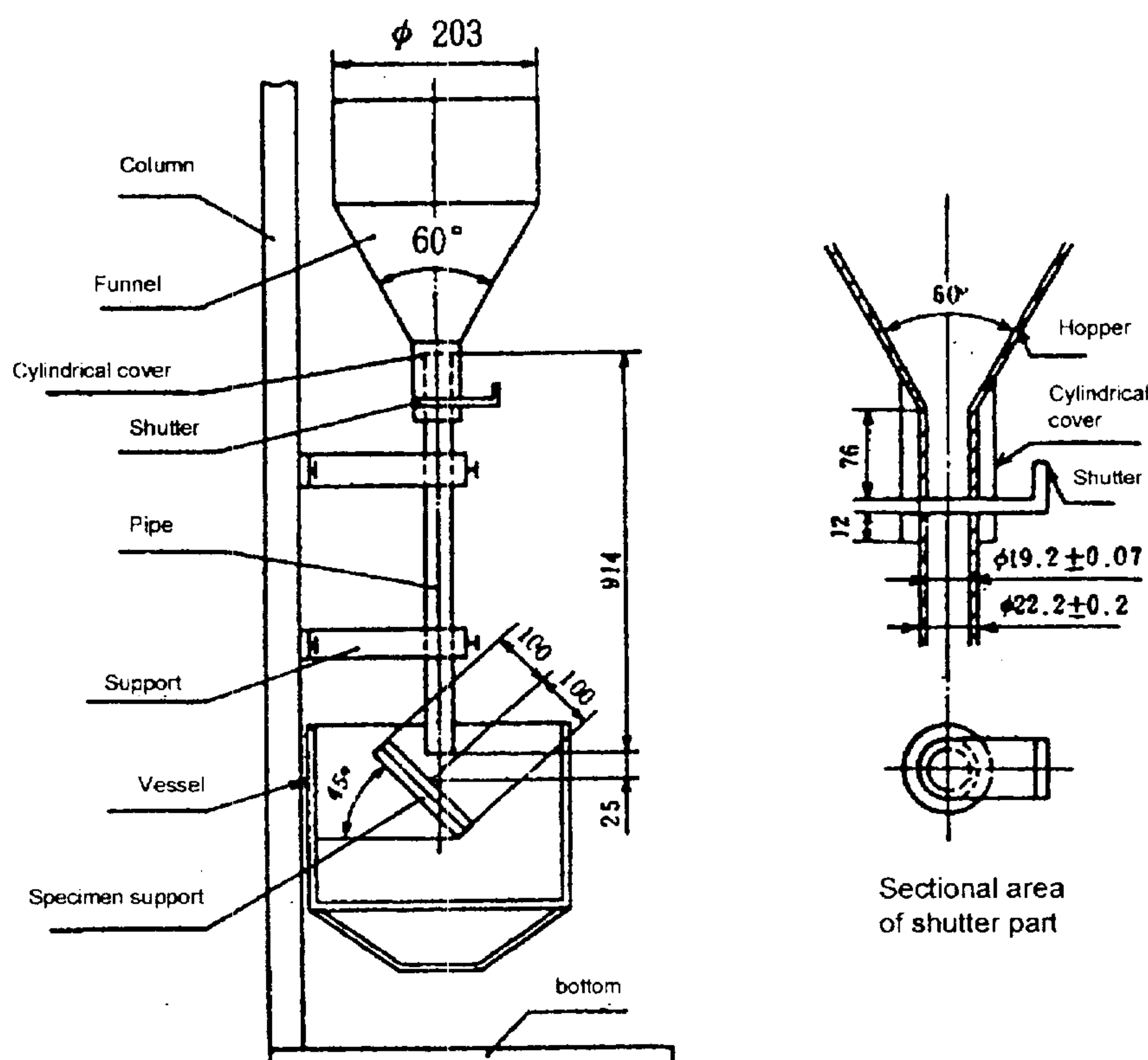
Figure 1. Sand fall abrasion tester
