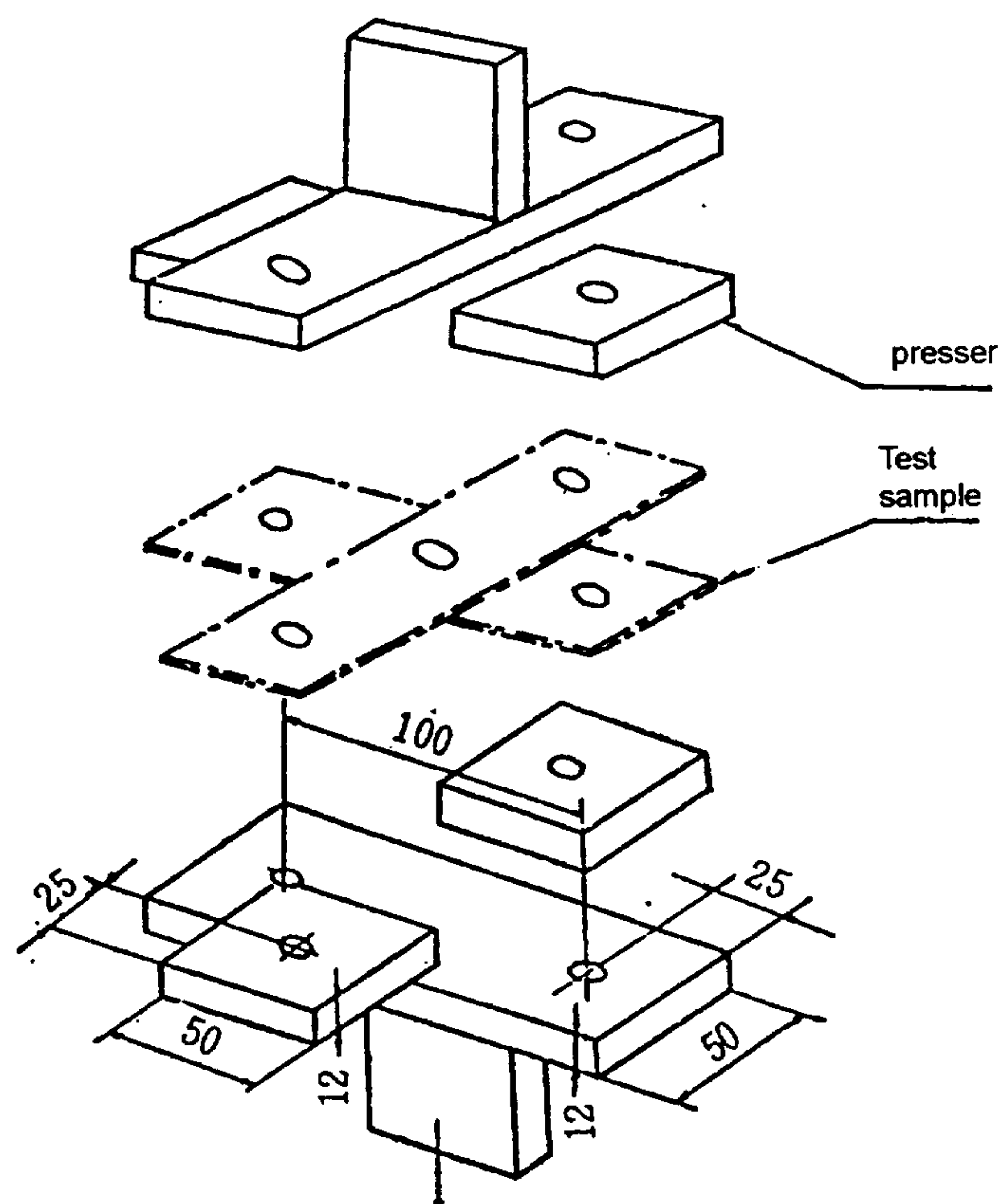
Fig : + type tension test jig (In case of less than 5 mm thickness)
