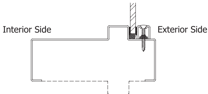
Optional Frame Member Section
