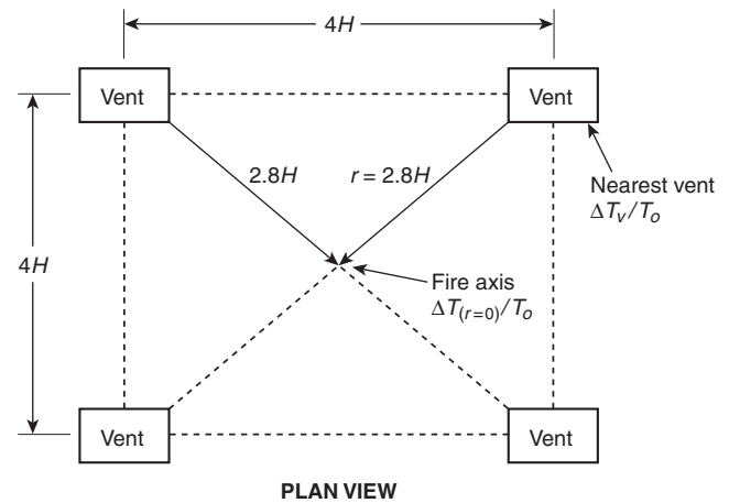
Figure A.5.4.2 Vent Spacing in Rectangular Matrix, When r = 2.8H , (\Delta T_v/T_0) = 0.5 ( \Delta T(r=0)/T_0 ) (plan view).
