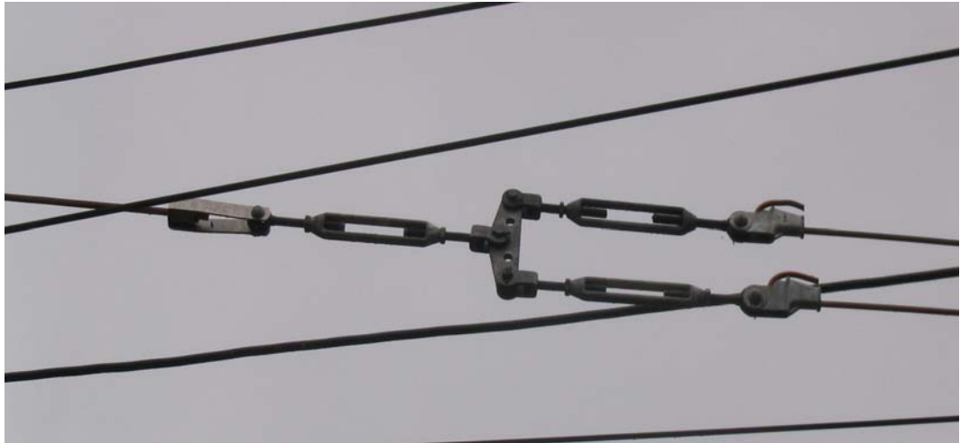
19/3.2mm tail wire with forked collar socket 121/544/022 fitted.
