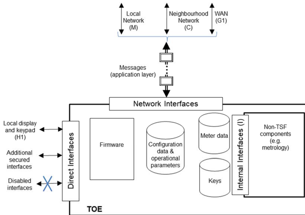
Figure 1 — Generic Smart Meter TOE Architecture
