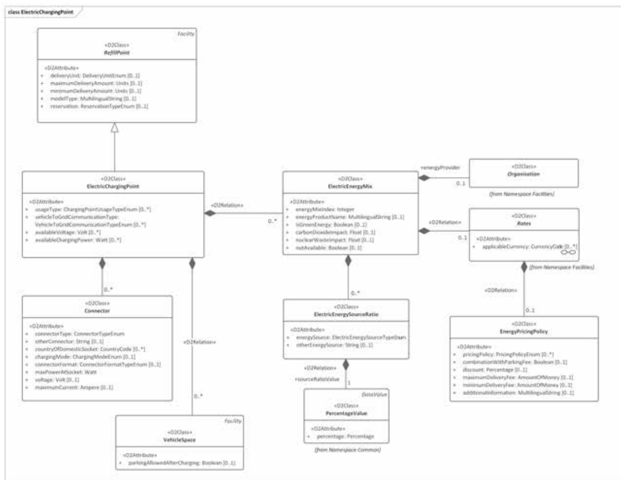
Figure 9 — ElectricChargingPoint class structure
