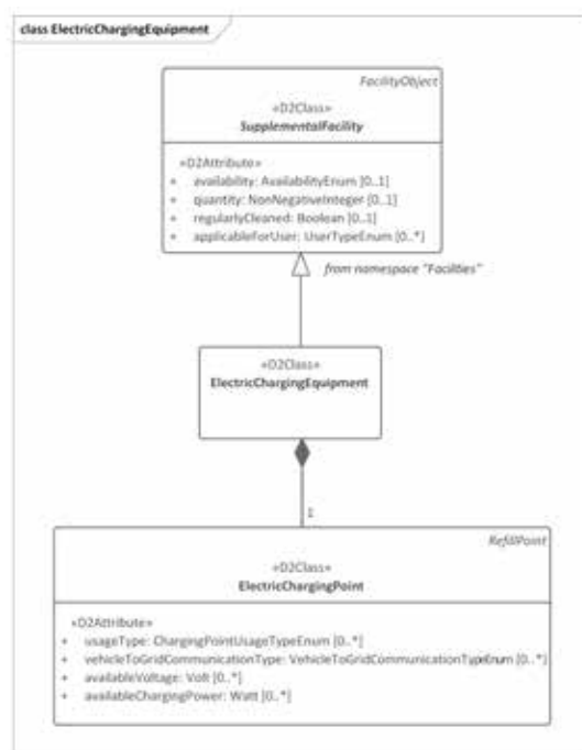
Figure 11 — Electric charging equipment
