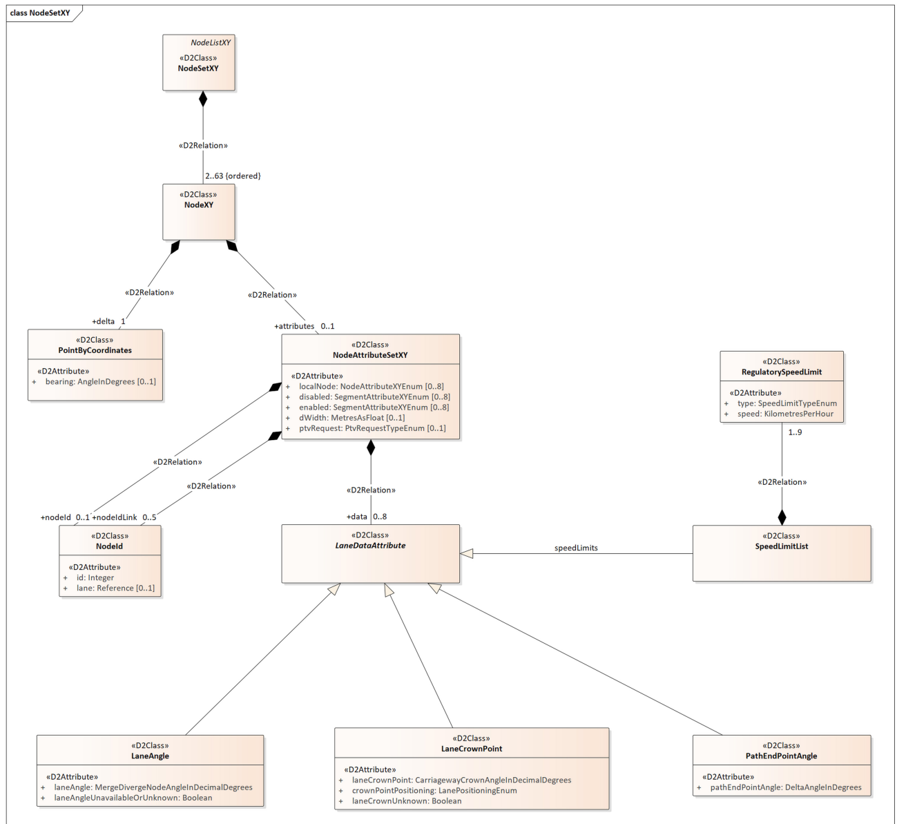
Figure 8 — “NodeSetXY” package class model
