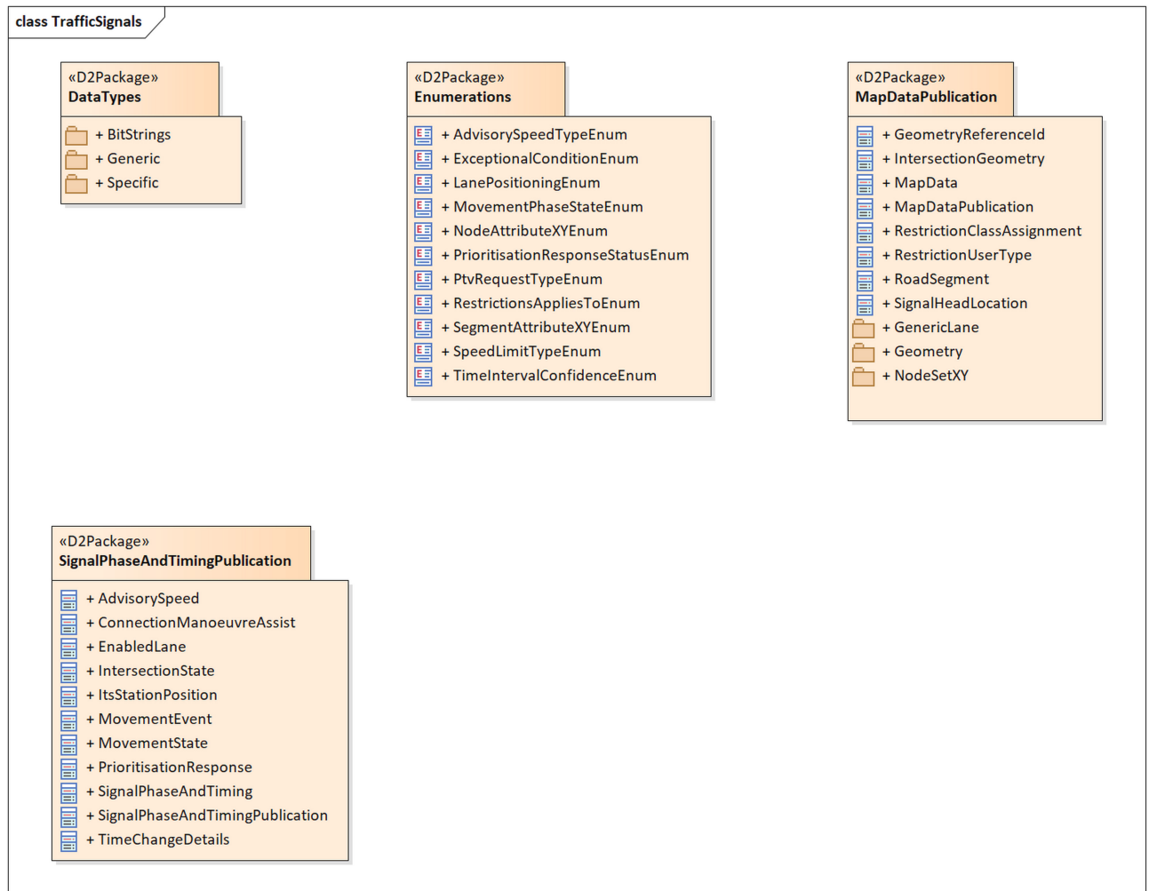
Figure 1 — The “TrafficSignals” package class model
