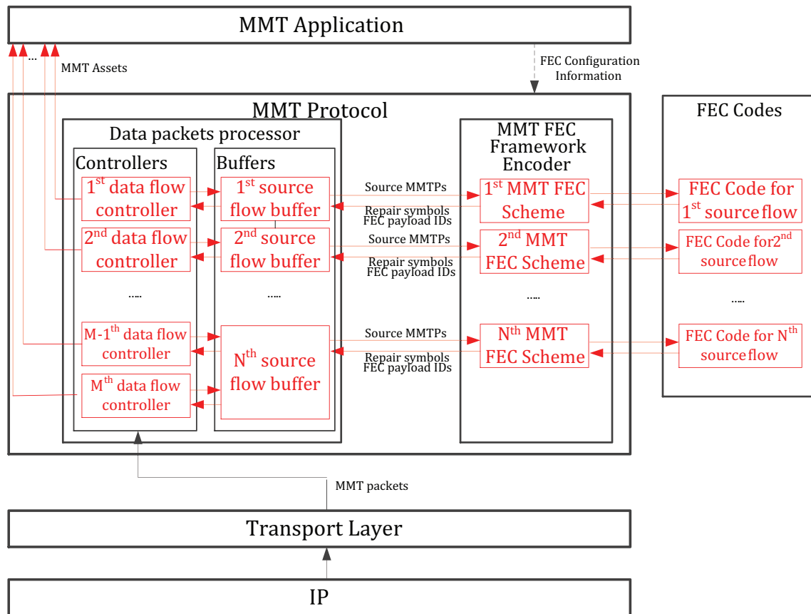
Figure 8 — Architecture for AL-FEC (MMT receiving entity)
