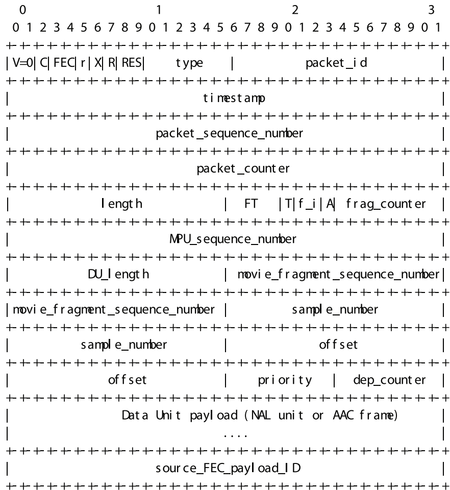
Figure 4 — MMTP packet
