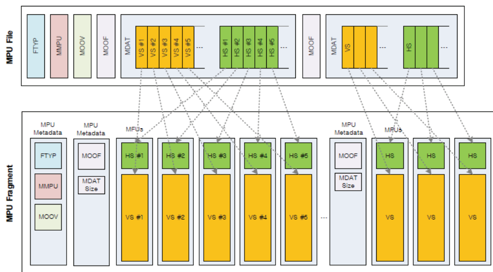
Figure 9 — MPU fragment building block
