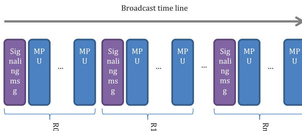
Figure 10 — Periodical signalling information transmission
