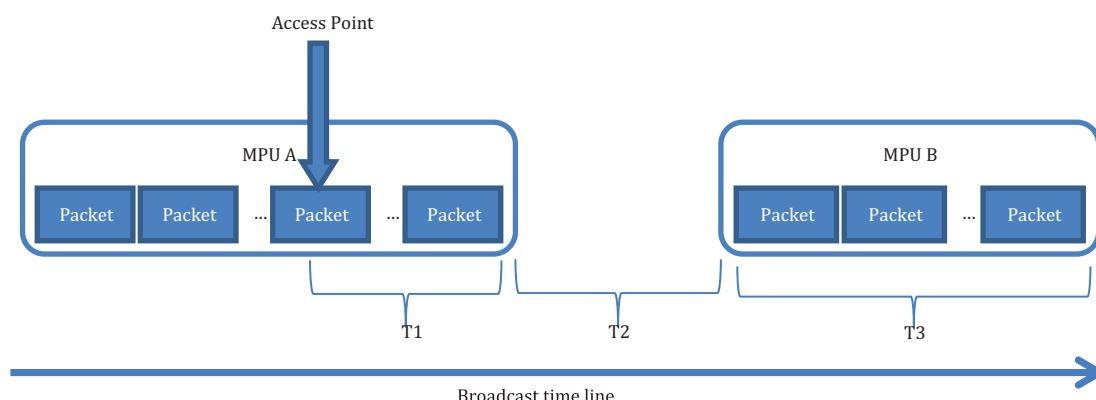
Figure 12 — Random access in the middle of MPU (case 1)
