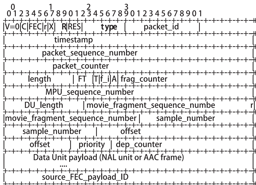
Figure 15 — Structure of MMTP packet
