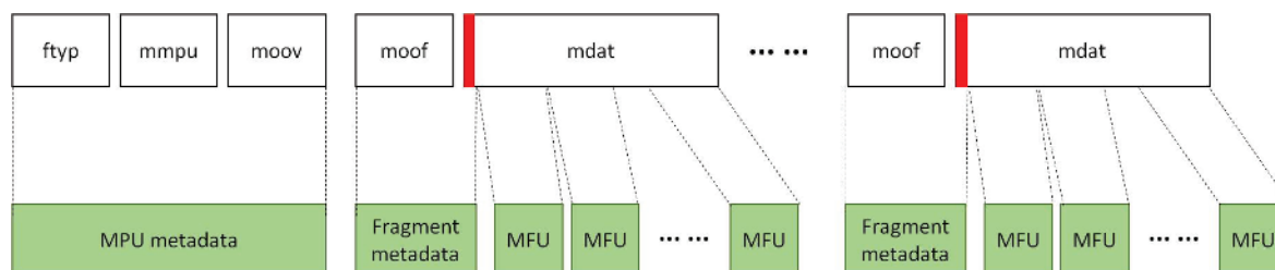
Figure 13 — MMTP Payload generation
