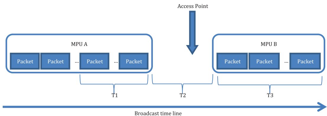
Figure 14 — Random access in the middle of Interval (case 2)
