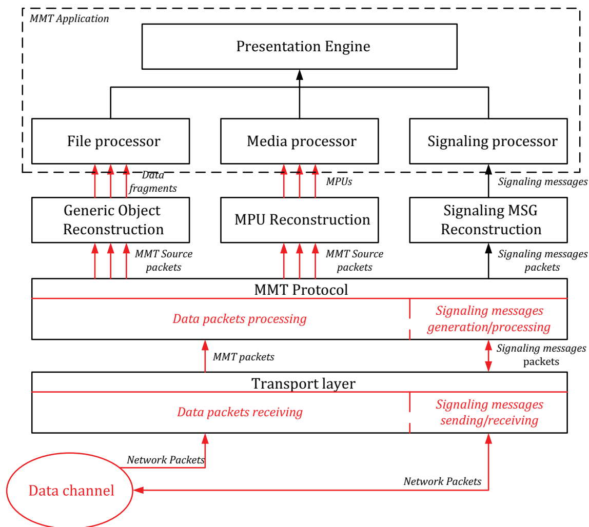
Figure 7 — MMT receiving entity structure
