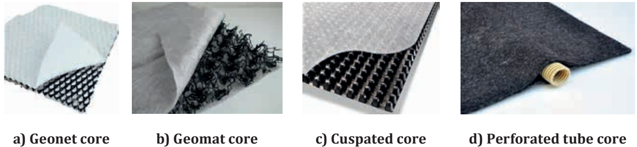
Figure 1 — Examples of drainage cores
