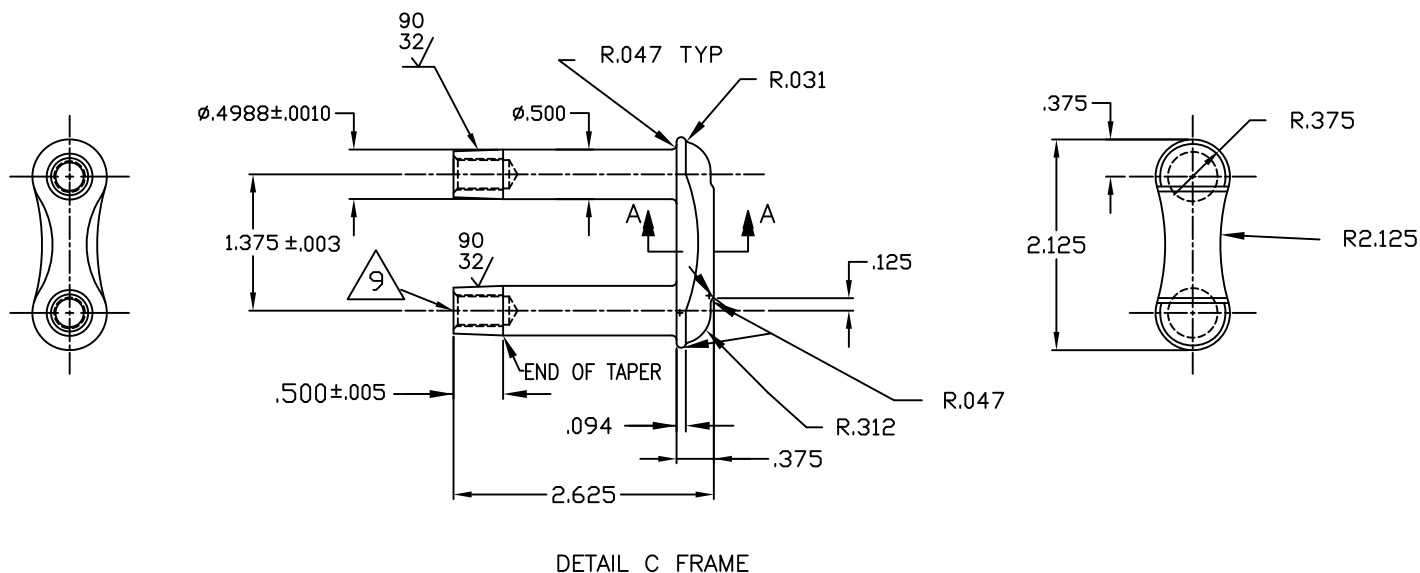
DETAIL C FRAME
