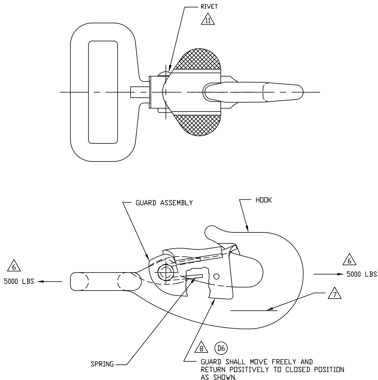
SNAP ASSEMBLY
