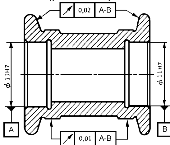
Figure 4 - Galet
