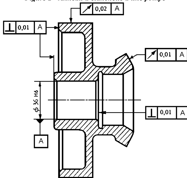
Figure 3 - Roue de friction
