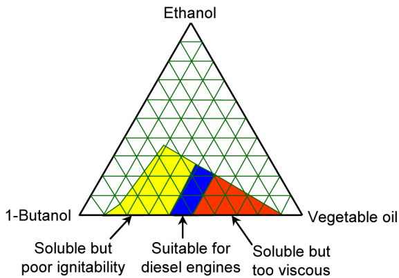
Fig. 3. Soluble and suitable ranges for high speed diesel engines of vegetable oil - 1-butanol - ethanol ternary blends
