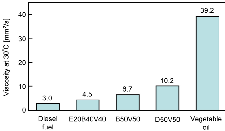
Fig. 2. Kinematic viscosities of the tested fuels and the vegetable oil in the blends at 30°C
