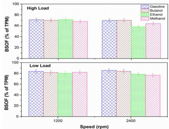
Figure 5. Variation in BSOF content of HCCI particulates for gasoline, butanol, ethanol and methanol.
