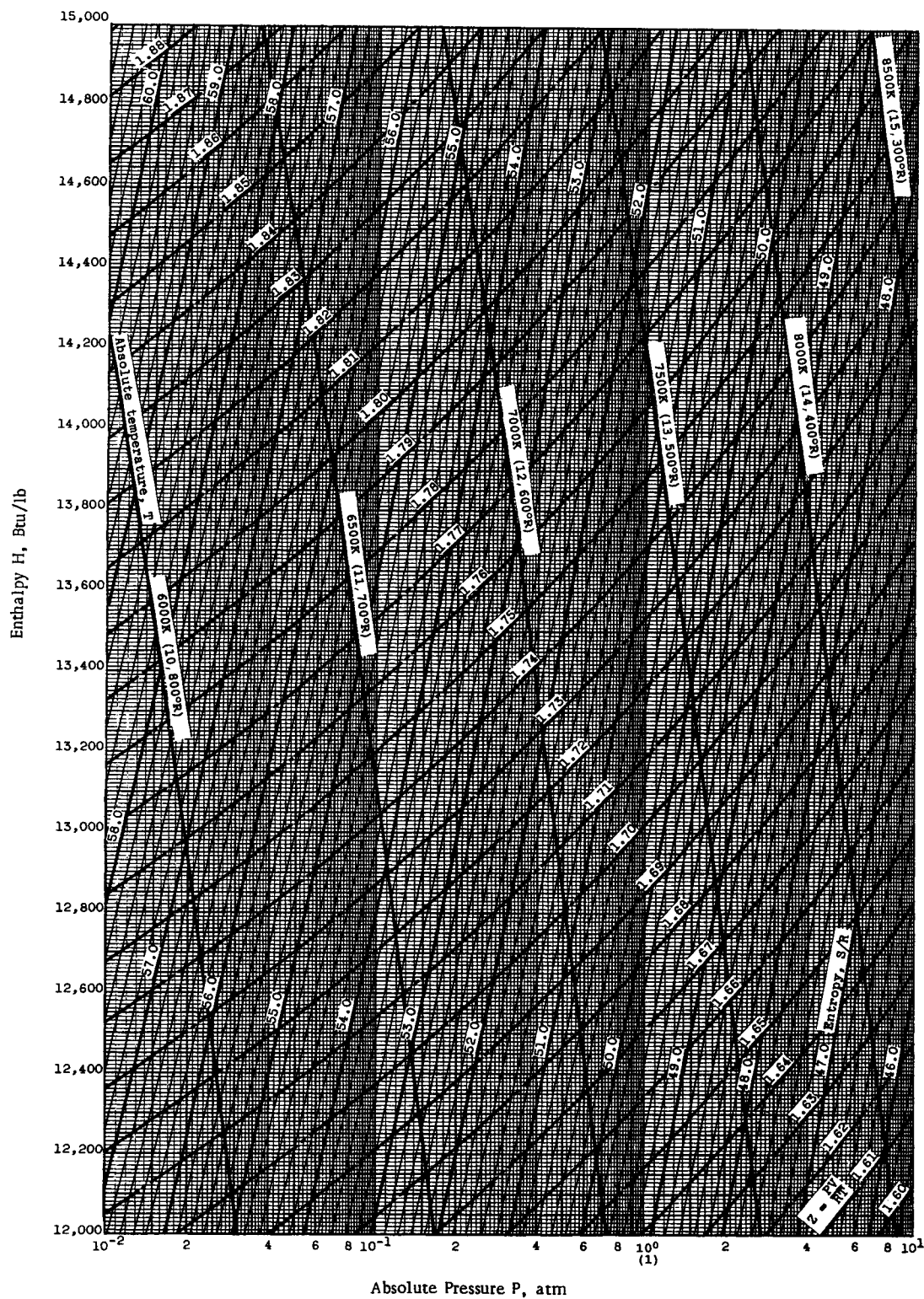
Figure 2E-12 - Chart 11 - Thermodynamic Chart For Air
