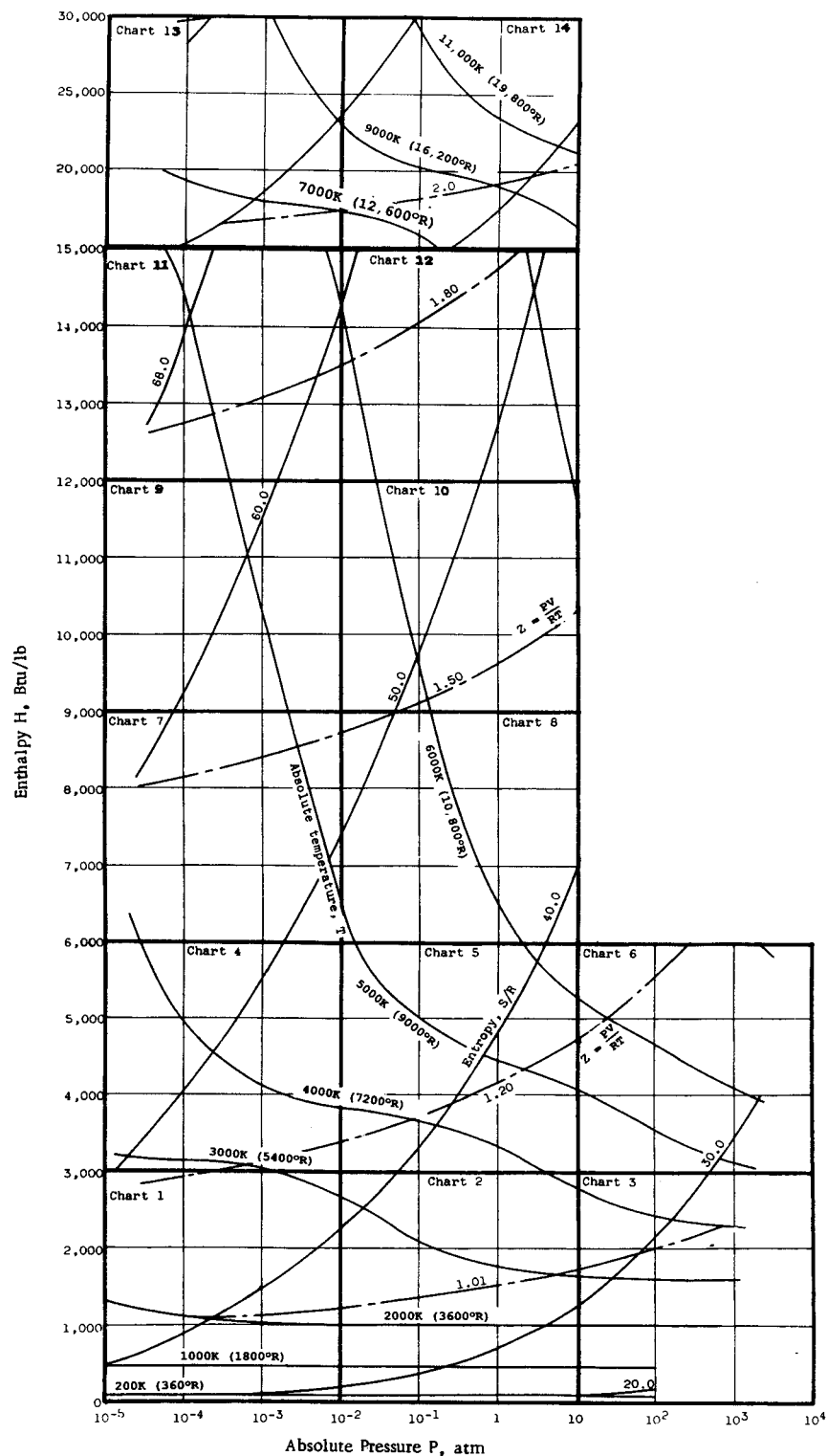
Figure 2E-1 - Pressure-Enthalpy Diagram for Air (Key to Charts); From NACA TN-4265
