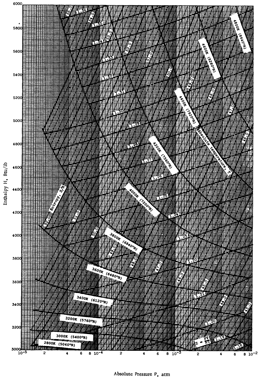
Figure 2E-5 - Chart 4 - Thermodynamic Chart For Air
