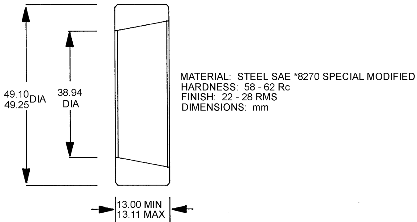
FIGURE B2 - RRTE Test Cylinder
