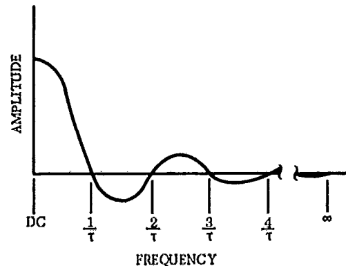
Figure 2. Pulse Train Frequency Spectrum
