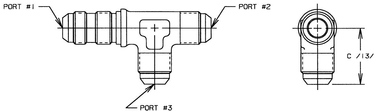
FIGURE 2 - FITTING, TEE, BULKHEAD END FOR OPTIONAL USE IN PORT NON-REDUCER SHOWN SAME AS FIGURE 1 EXCEPT AS SHOWN
