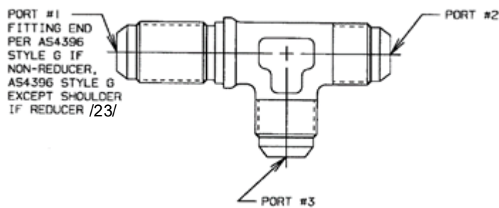
FIGURE 4 - FITTING, TEE, BULKHEAD END NOT FOR USE IN PORT NON-REDUCER SHOWN SAME AS FIGURE 2 EXCEPT AS SHOWN /21/ BULKHEAD END NOT FOR USE IN PORT
