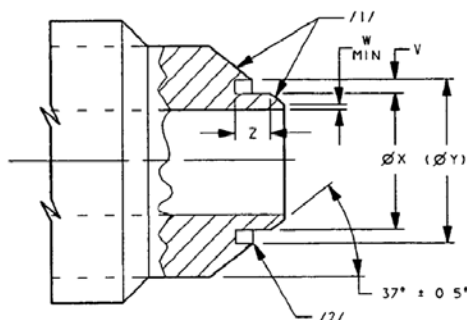
FIGURE 3 – ENLARGED VIEW A FROM FIGURES 1 AND 2
