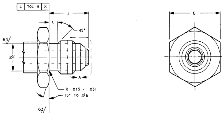
FIGURE 2 – FITTING END, SEAL RING, STYLE E
