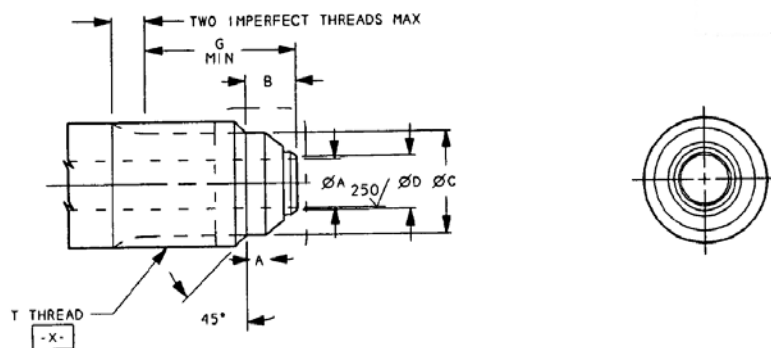
FIGURE 1 – FITTING END, SEAL RING, STYLE G
