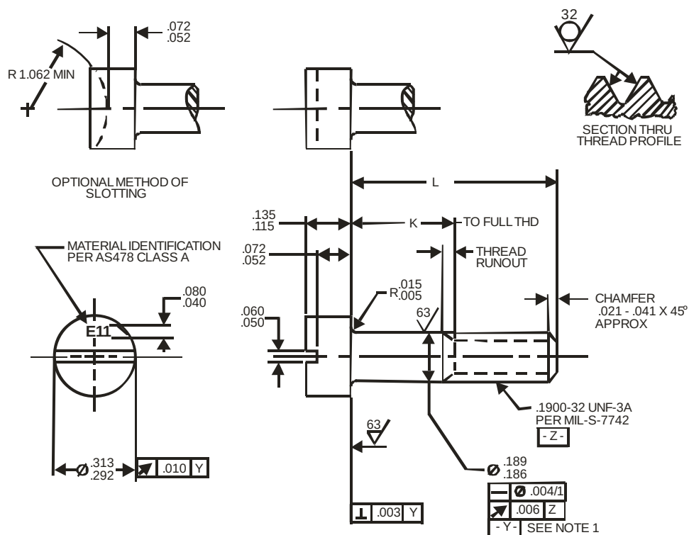
FIGURE 1 - SCREW
