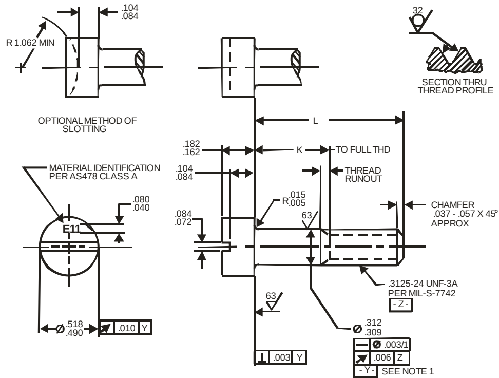
FIGURE 1 – SCREW
