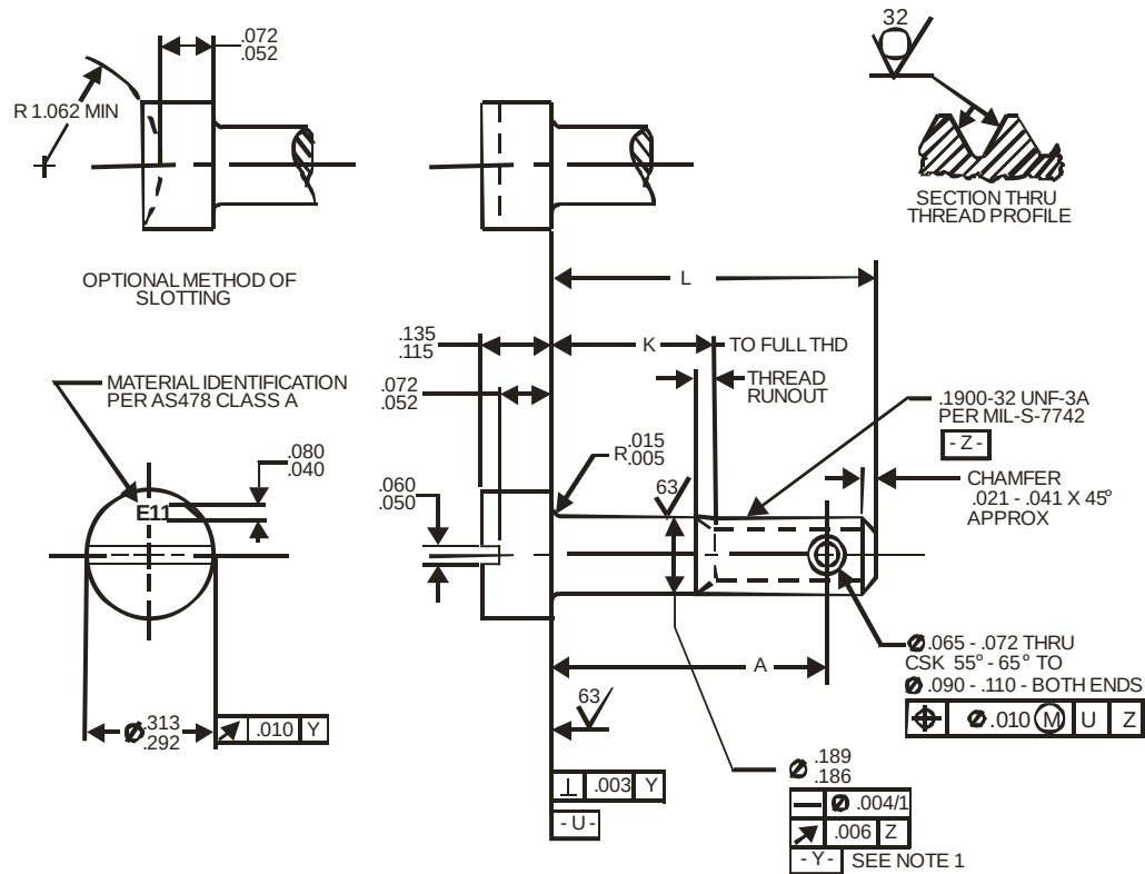
FIGURE 1 - SCREW
