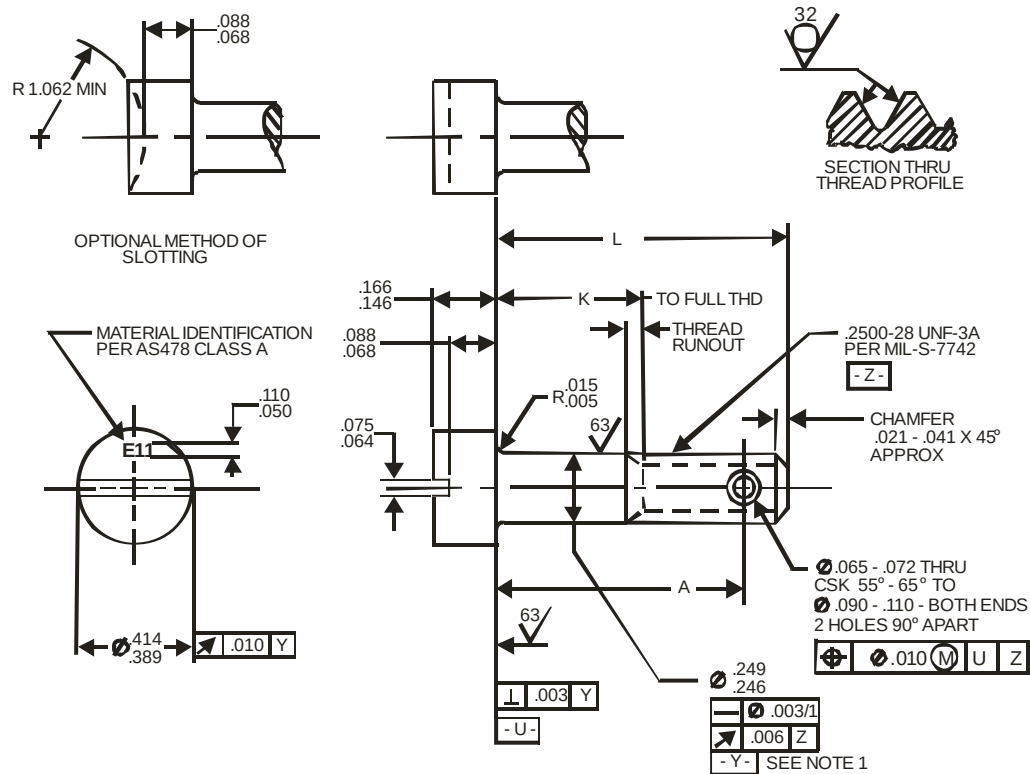
FIGURE 1 – SCREW
