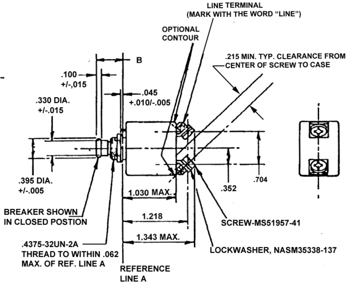
FIGURE 1 - CIRCUIT BREAKER CONFIGURATION AND DIMENSIONS
