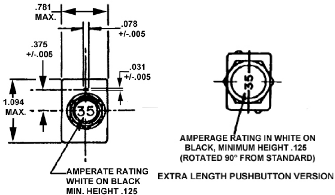
FIGURE 1 - CIRCUIT BREAKER CONFIGURATION AND DIMENSIONS (CONTINUED)
