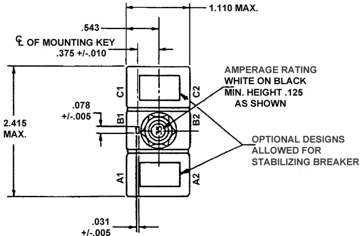
FIGURE 1 - TRIP-FREE CIRCUIT BREAKER
