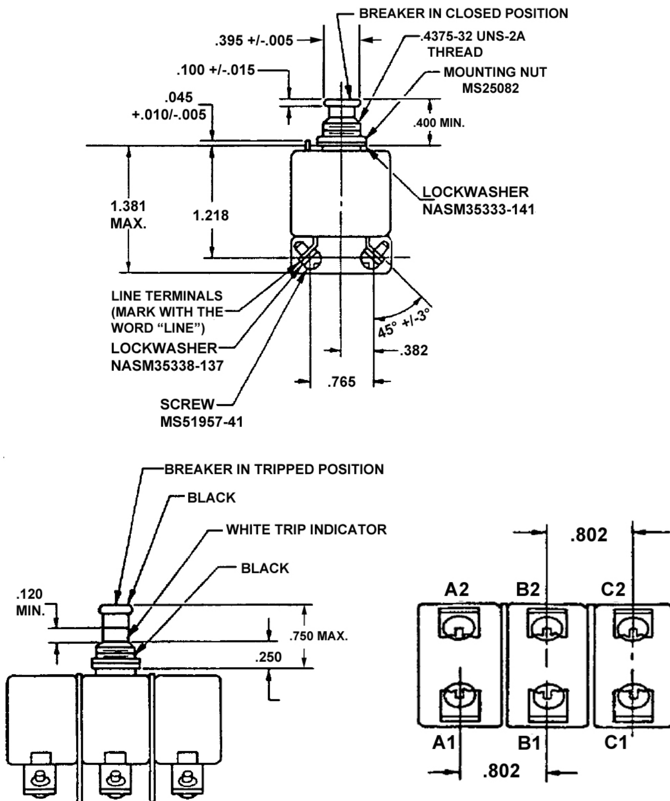
FIGURE 1 - TRIP-FREE CIRCUIT BREAKER (CONTINUED)
