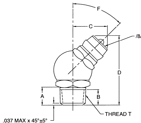
FIGURE 2 - FITTING, ELBOW
