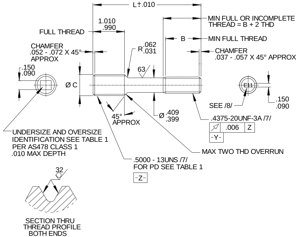
FIGURE 1 - STUD
