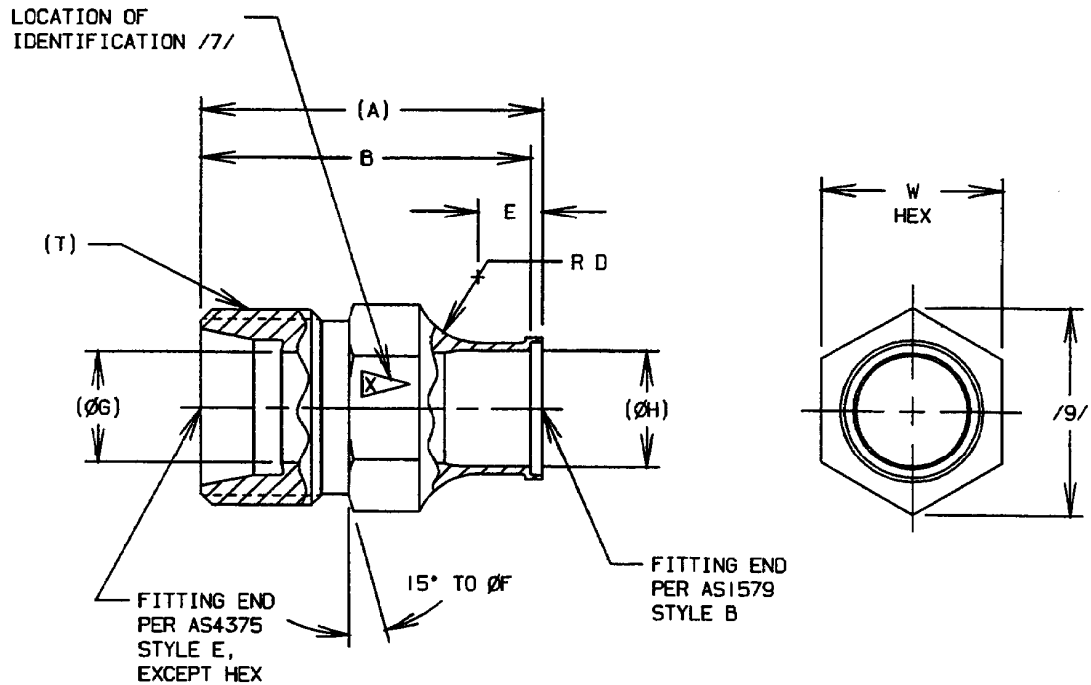
FIGURE 1 - FITTING, ADAPTER
