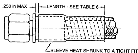
FIGURE 2 - SPIRAL AND POYESTER ABRASION COVER /7/, /8/
