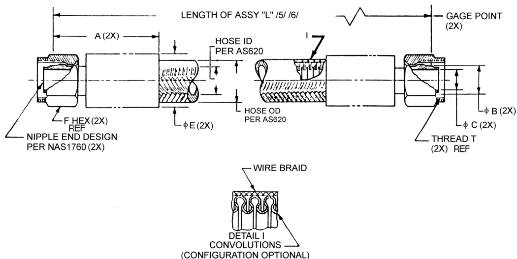
FIGURE 1 - HOSE ASSEMBLY
