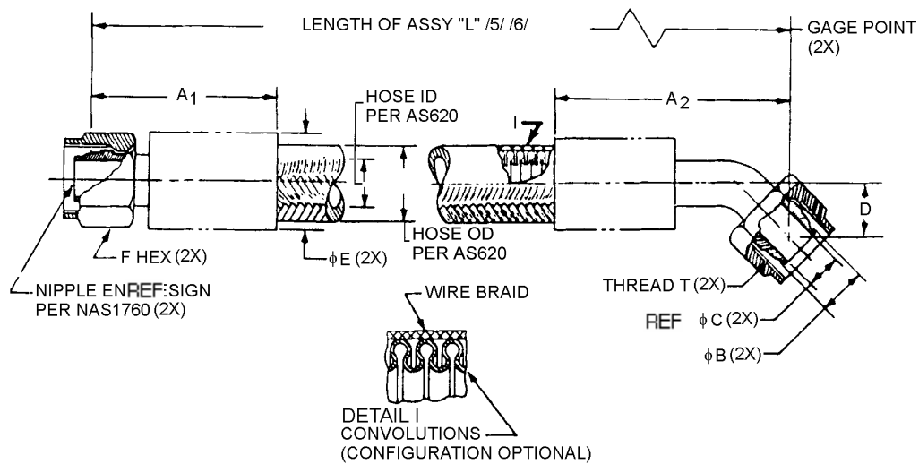
FIGURE 1 - HOSE ASSEMBLY
