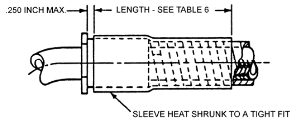
FIGURE 2 - SPIRAL AND POYESTER ABRASION COVER /6/, /7/
