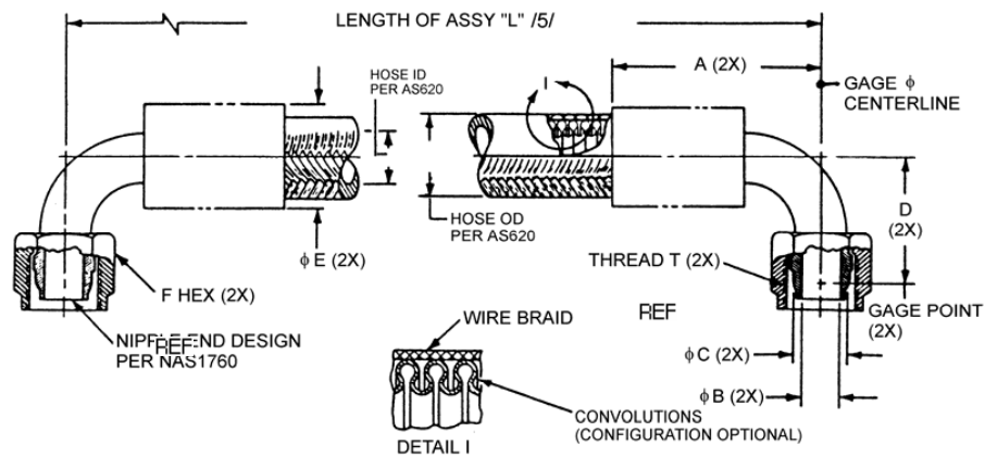
FIGURE 1 - HOSE ASSEMBLY
