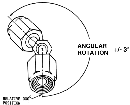
FIGURE 3 - FITTING ANGULAR ORIENTATION /15/
