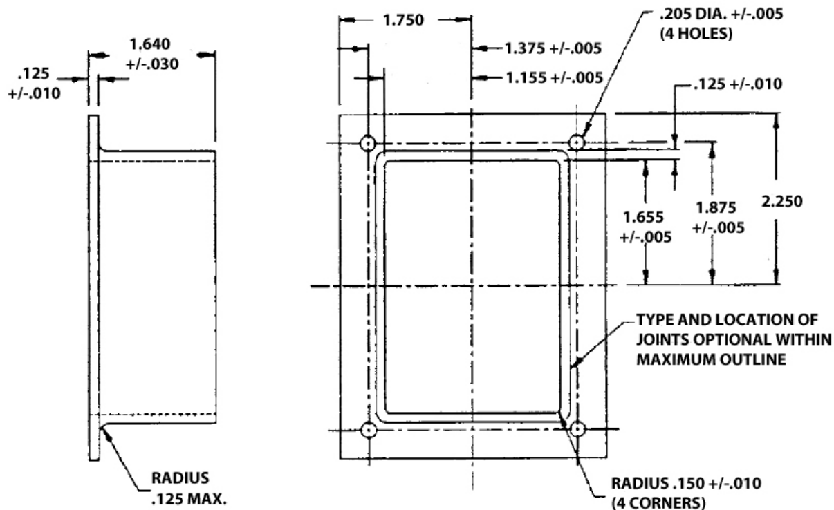
FIGURE 1 - SHIELD CONFIGURATION
