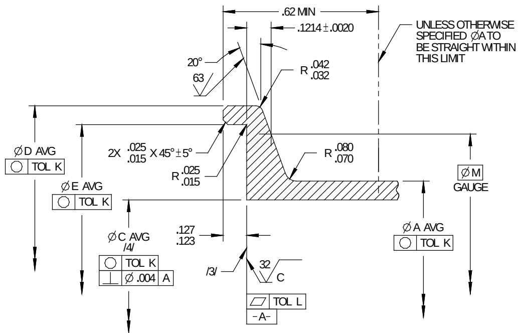
FIGURE 1 - FLANGE END DESIGN
