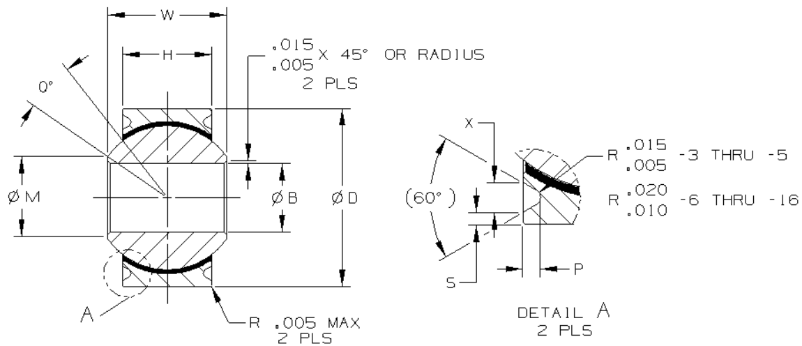
FIGURE 1 – PART CONFIGURATION
