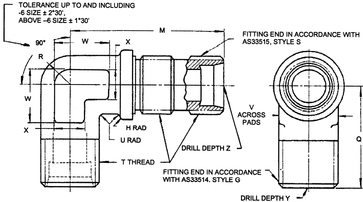
FIGURE 1 - ELBOW, BULKHEAD UNIVERSAL 90°, FLARELESS TUBE
