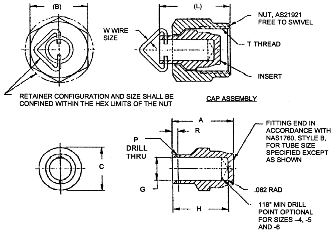
FIGURE 1 - CAP, PRESSURE SEAL, FLARELESS TUBE FITTING /14/
