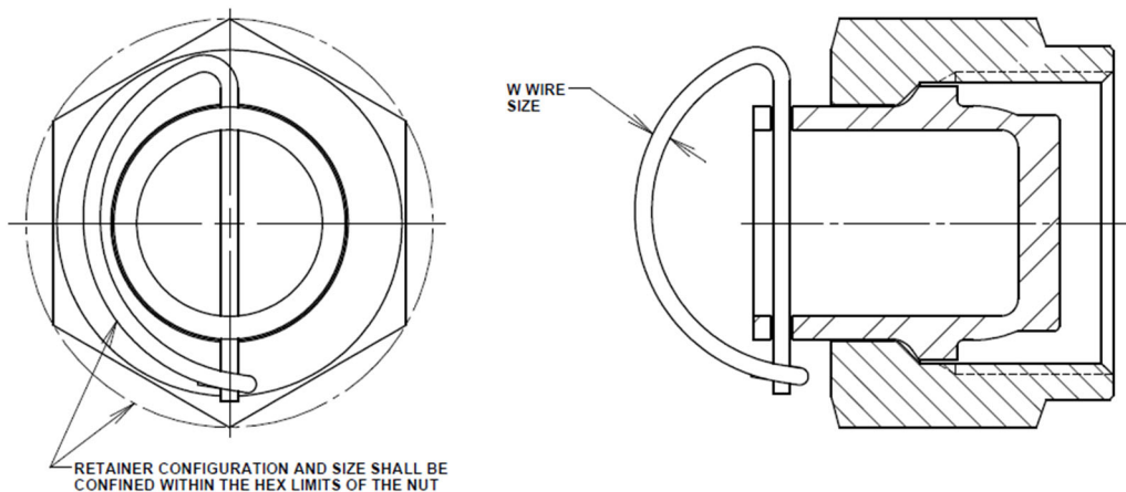
FIGURE 2 - ALTERNATIVE WIRE DESIGN FOR CAP ASSEMBLY /14/
