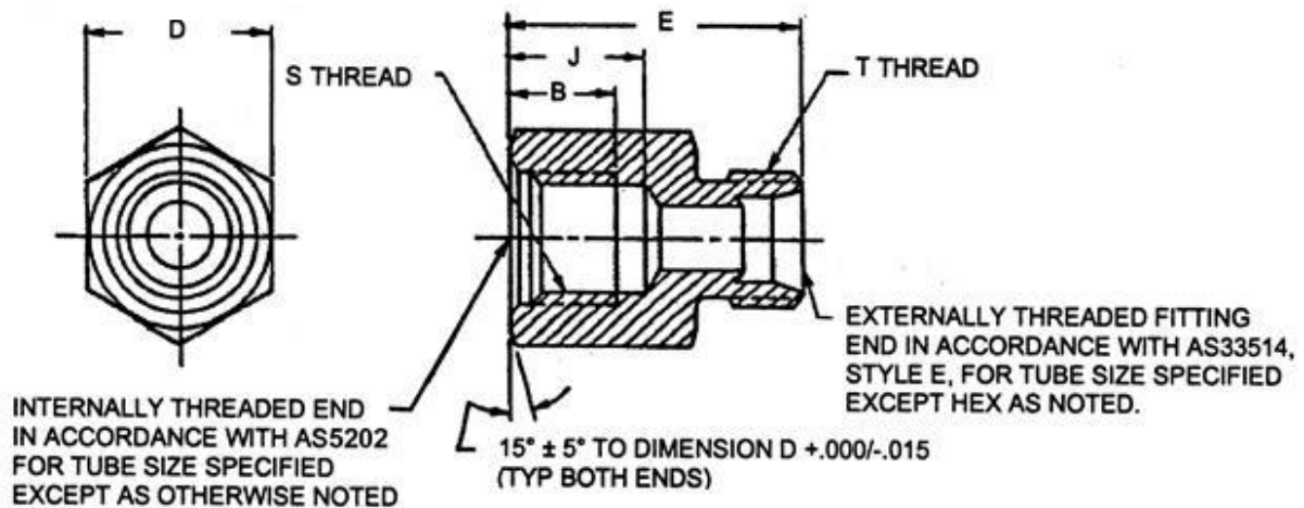
FIGURE 1 - ADAPTER, STRAIGHT, TUBE TO BOSS
