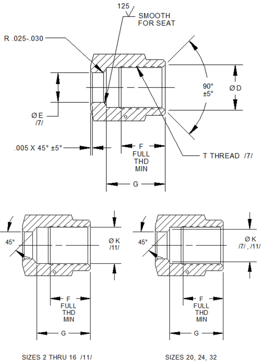
VIEWS SHOWING DIM K CONFIGURATION FOR VARIOUS SIZES
