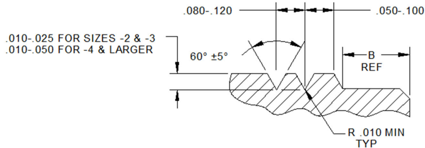
VIEW A TITANIUM PARTS ONLY
