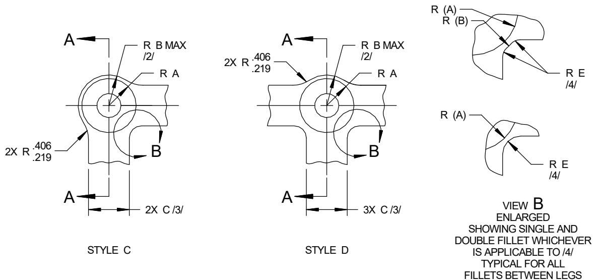
FIGURE 2 - CONTOUR AND MOUNTING END, STYLES C AND D
