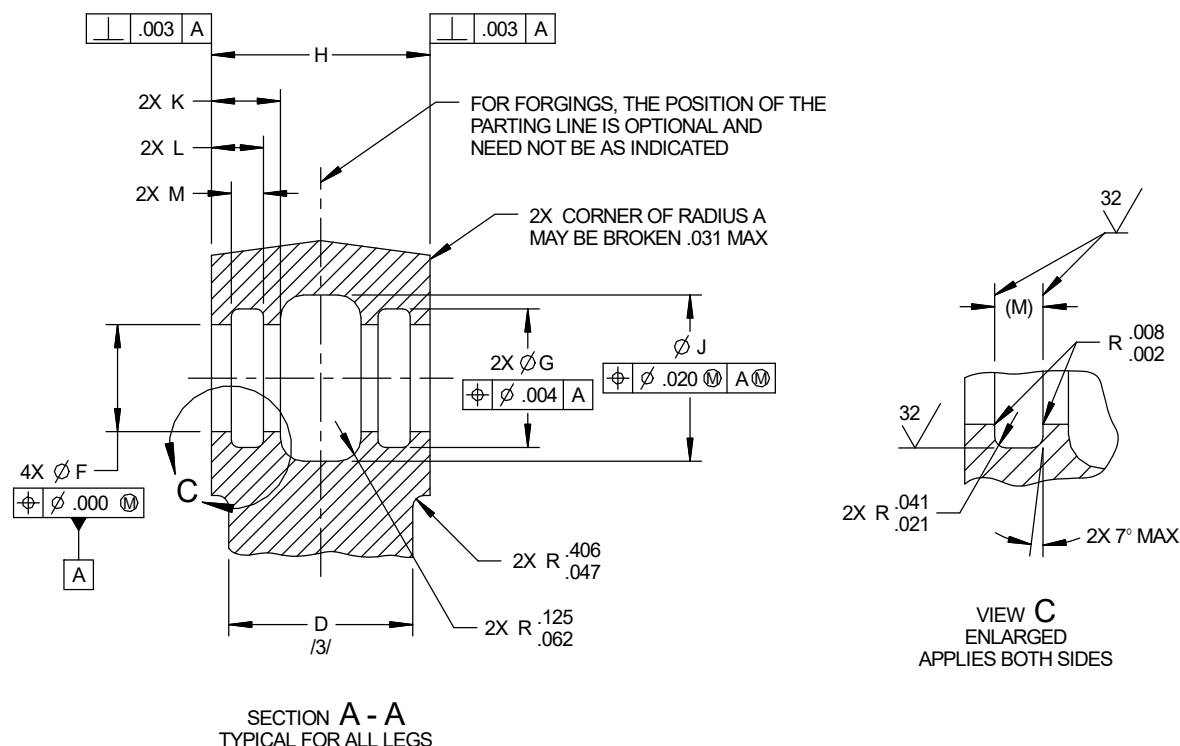
FIGURE 3 - CONTOUR AND MOUNTING END, CROSS SECTION
