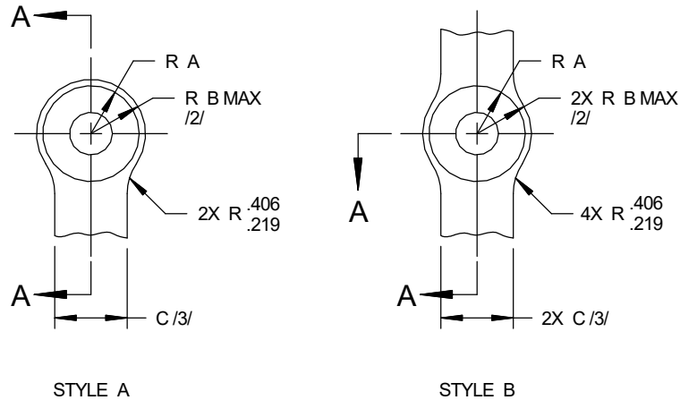
FIGURE 1 - CONTOUR AND MOUNTING END, STYLES A AND B
