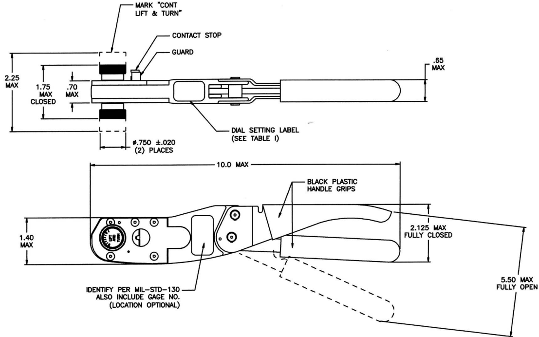
FIGURE 1 – M22520/17 TOOL
